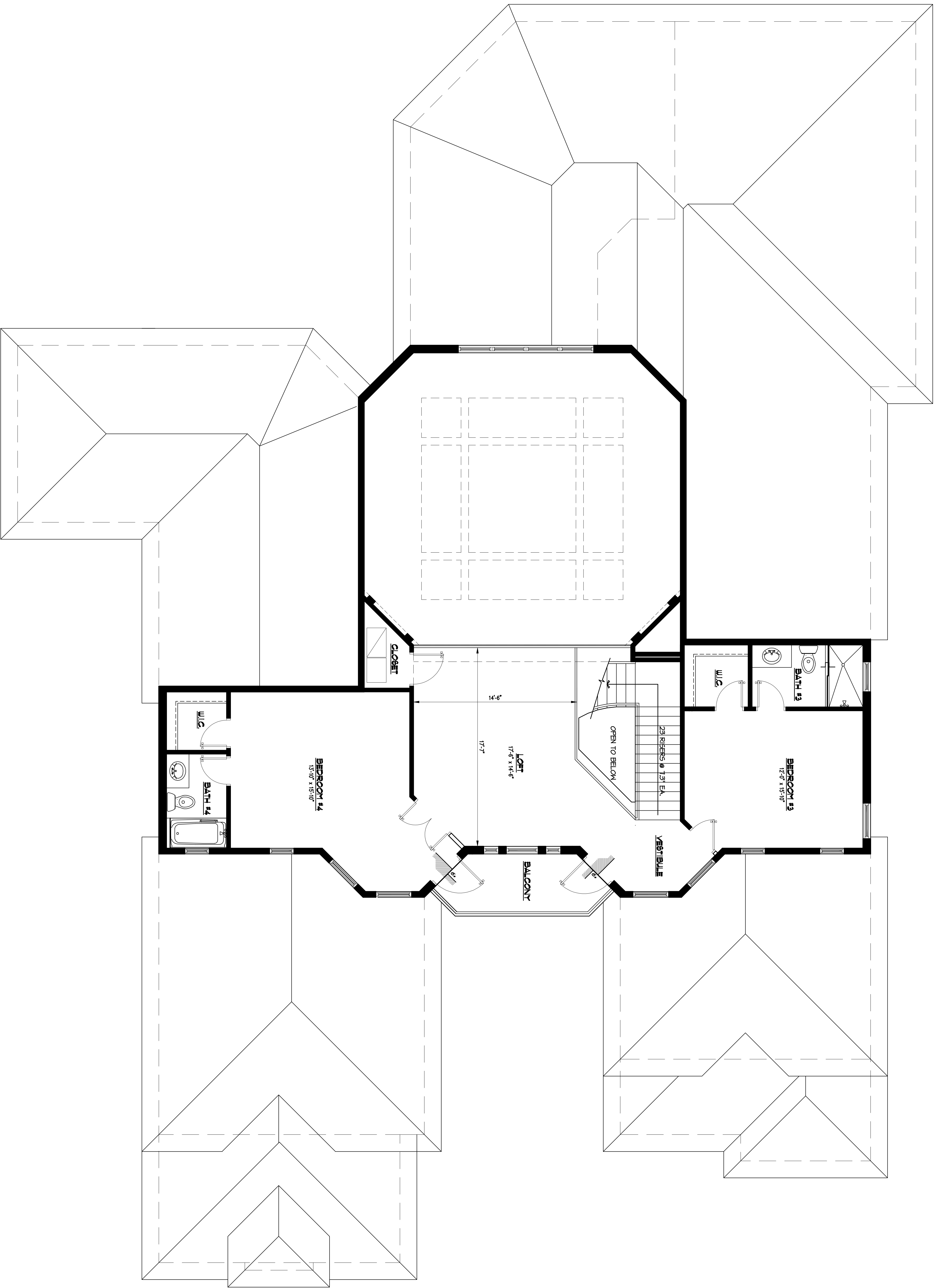
SECOND FLOOR PLAN SCALE 1/4" = 1'-0"
